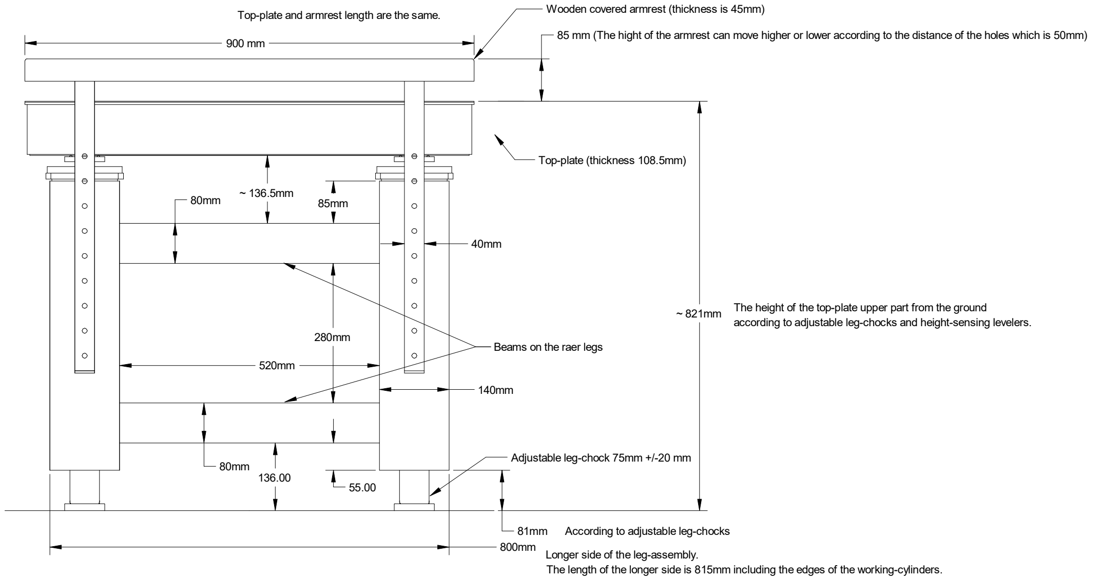
Front side of the leg-assembly with top-plate and wooden-armrest from the front view
