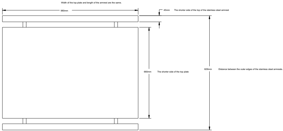
Top plate upper view with 2 stainless steel armrests
