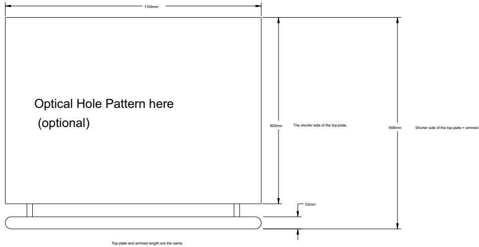
1100 x 800 mm table: Top-plate with armrest upper view
